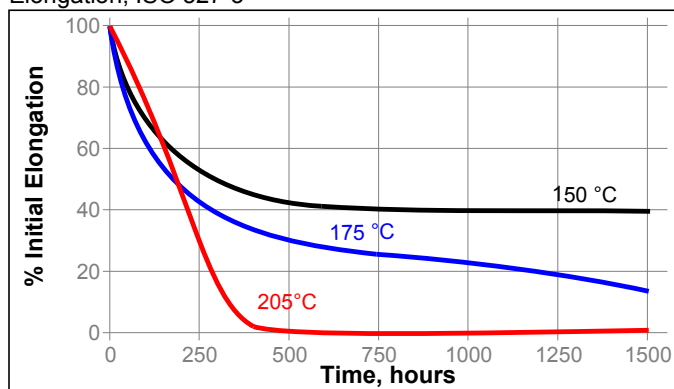
Elongation, ISO 527-3
